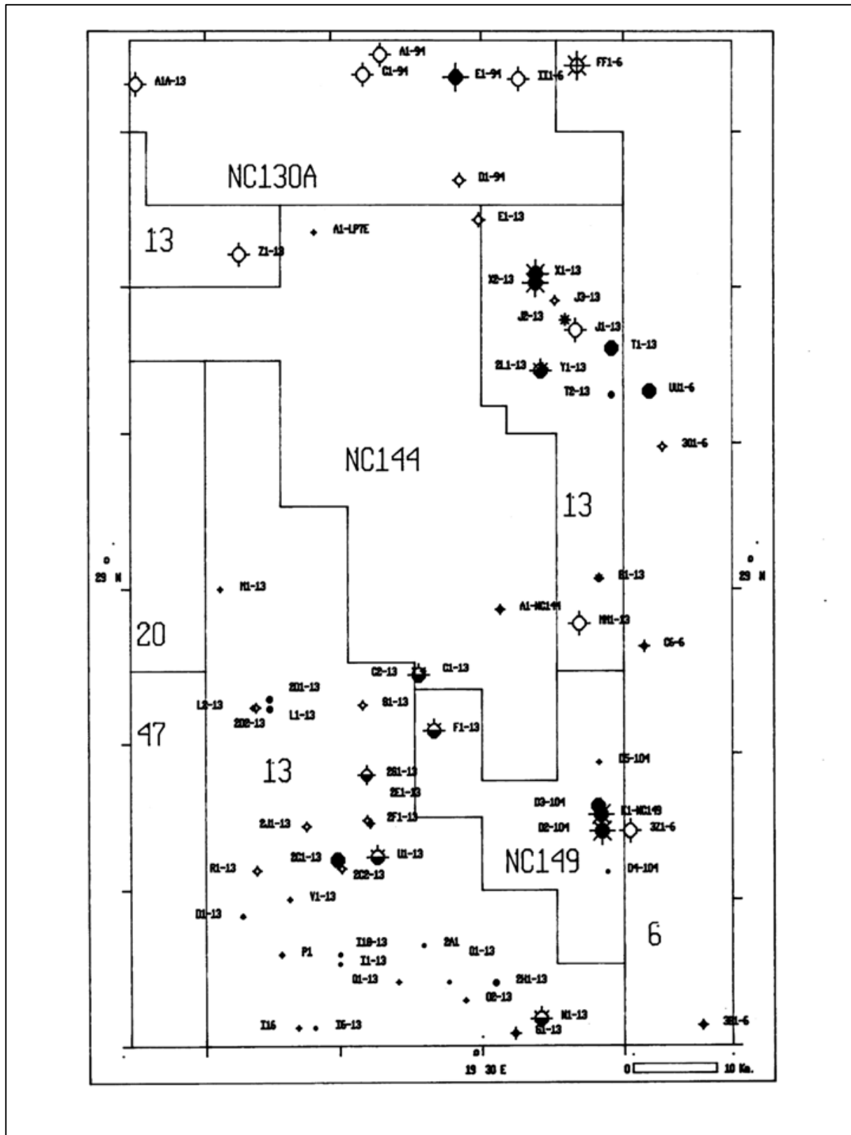
Figure1. Well location map of Hagfa Trough, Central Sirte Basin, Libya. The size of well symbols corresponds to the statistical significance of geothermal gradients BHT data and corresponding extrapolated surface temperature intercepts of the well.
