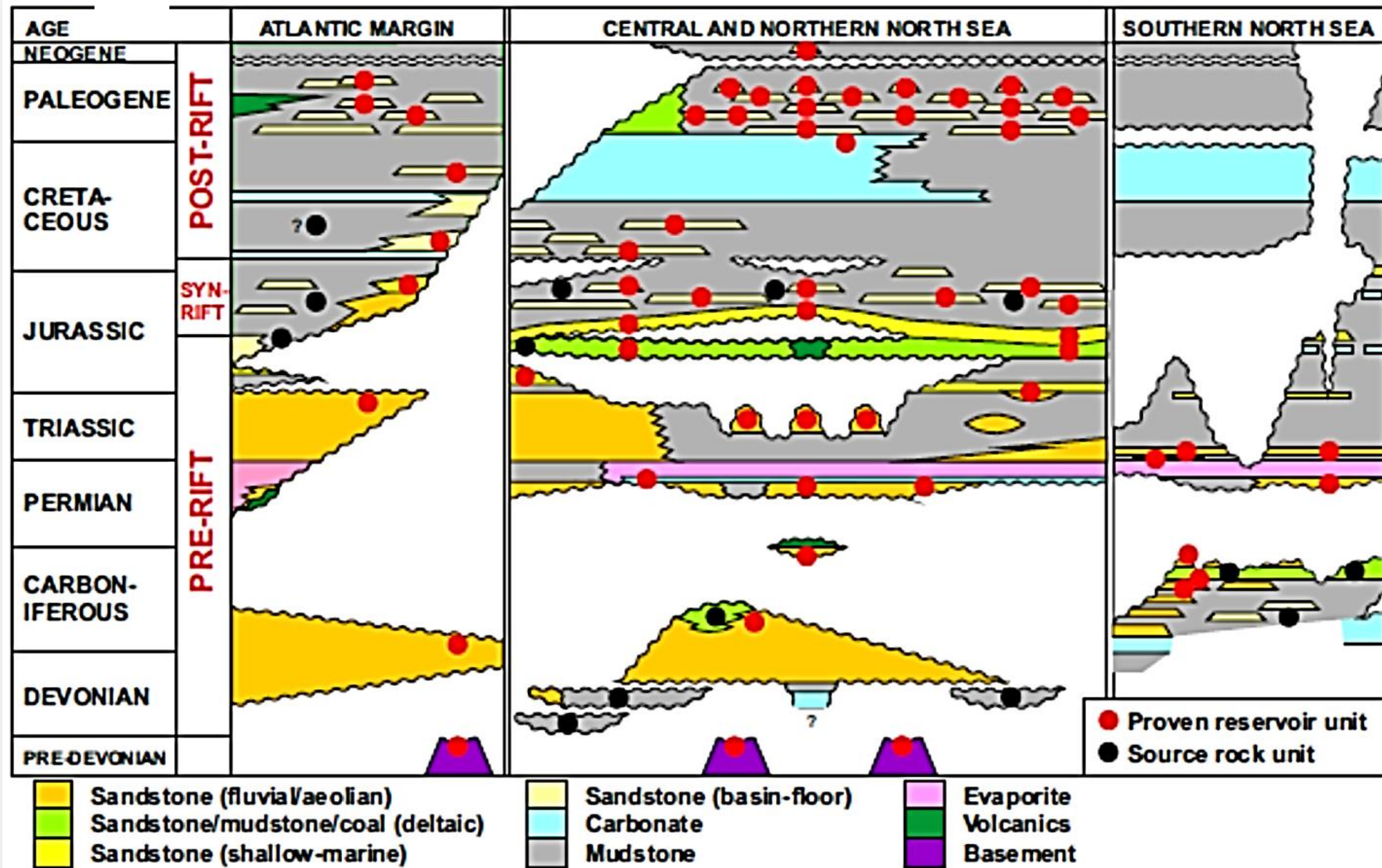
Simplified stratigraphy and lithofacies in UKCS oil and gas basins
